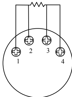
Example 4-Wire RTD Configuration.
