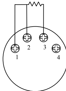
Sensor Connections
