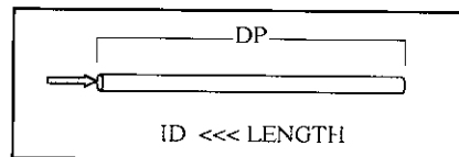
Figure 3. Application of Hagen-Poiseuille Law.
