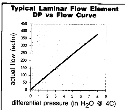
Figure 2. Typical calibration curve for laminar flow element.
